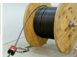
RM35 with RUNPOLIFTER L1 600 and 3 x 35 mm² cable
