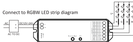
Connect to RGB+CCT LED strip diagram
